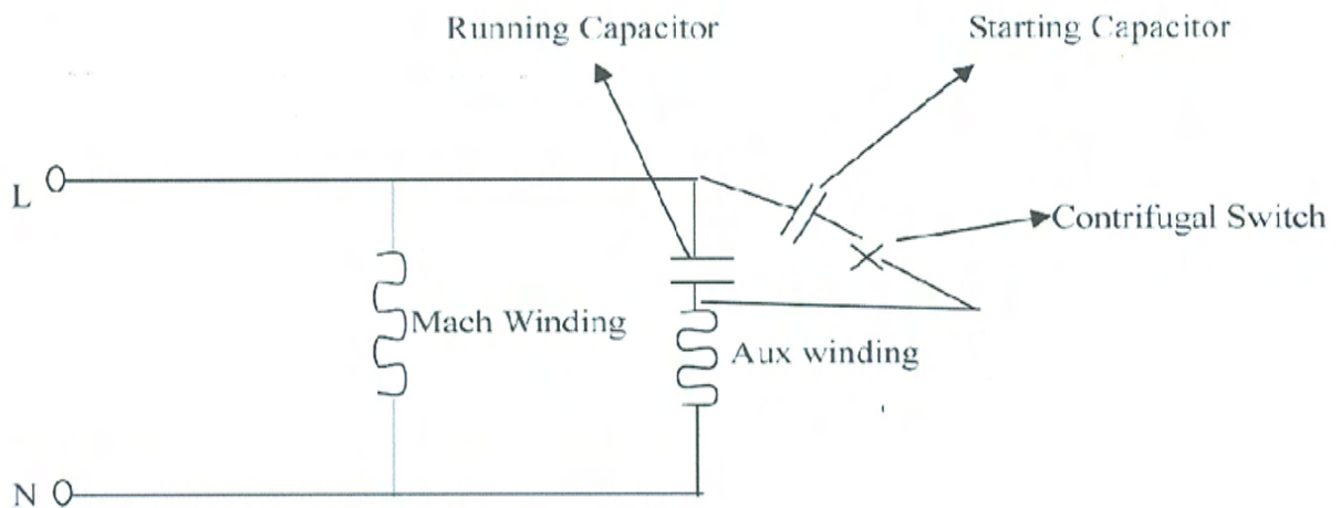
Schematics of motor
