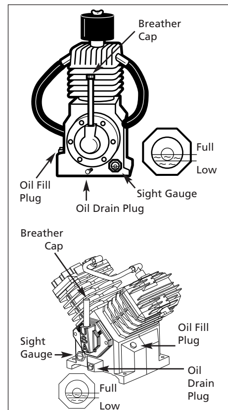
Figure 3 - Oil Fill Diagram
