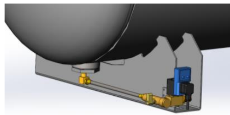
Channel Feet
